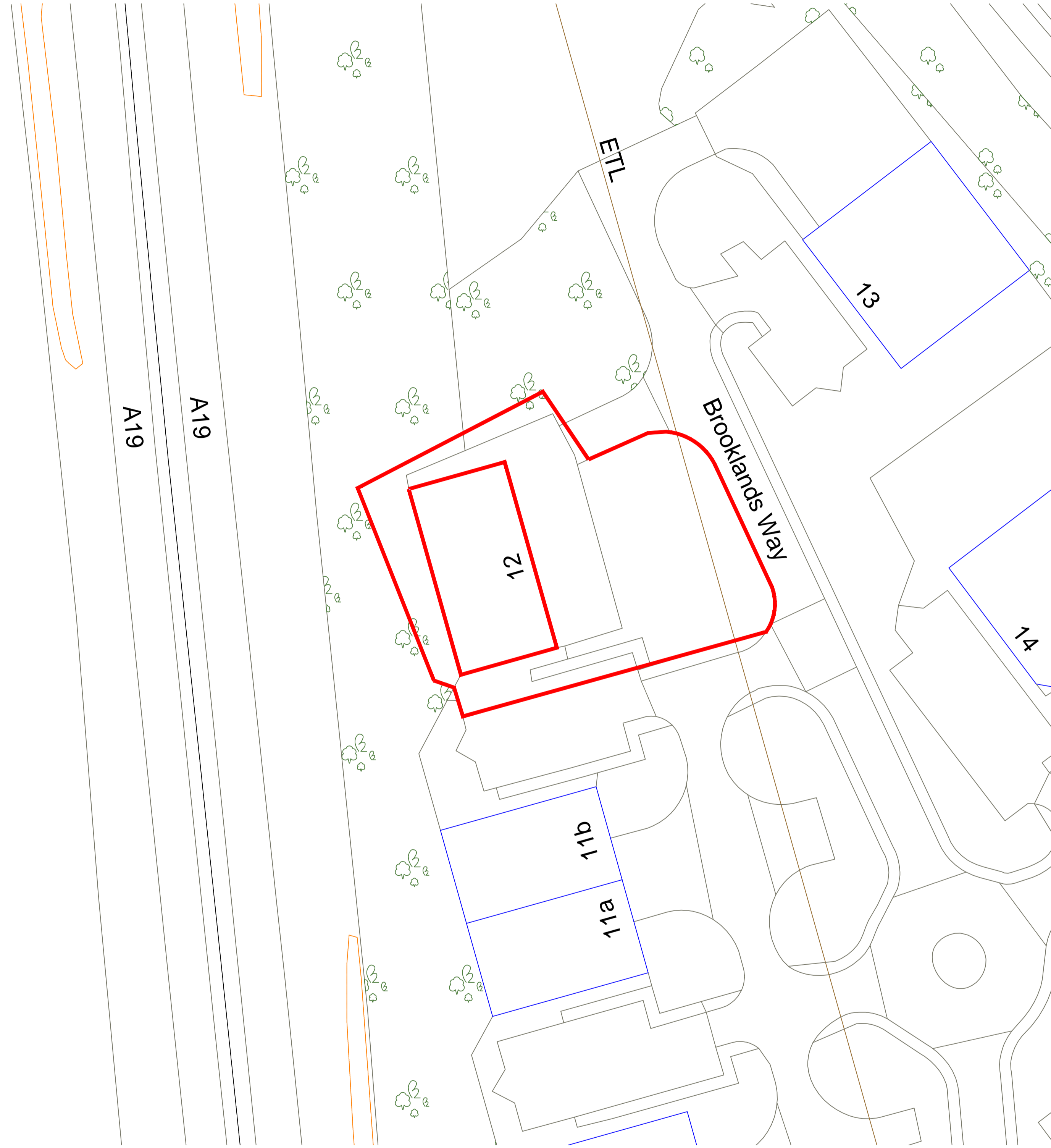
Block Plan - 1:500
